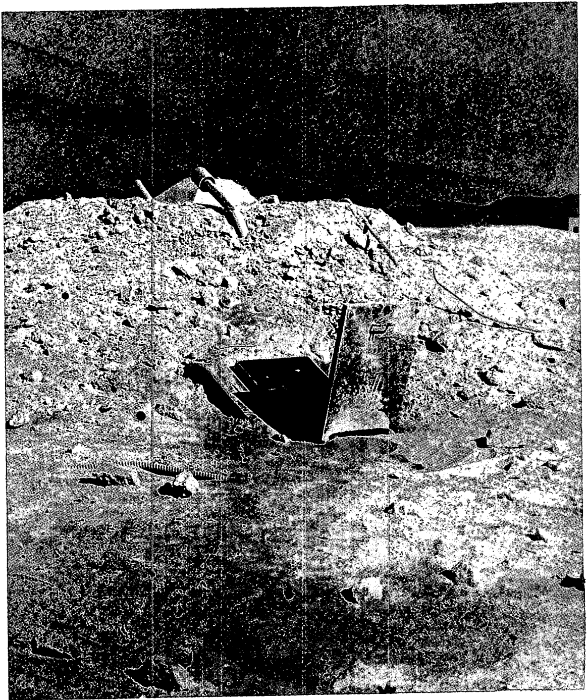
Fig. 7—Family-shelter ventilators bent over by blast.
